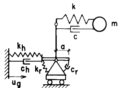
Fig. 1 Soil-structure model [14]
