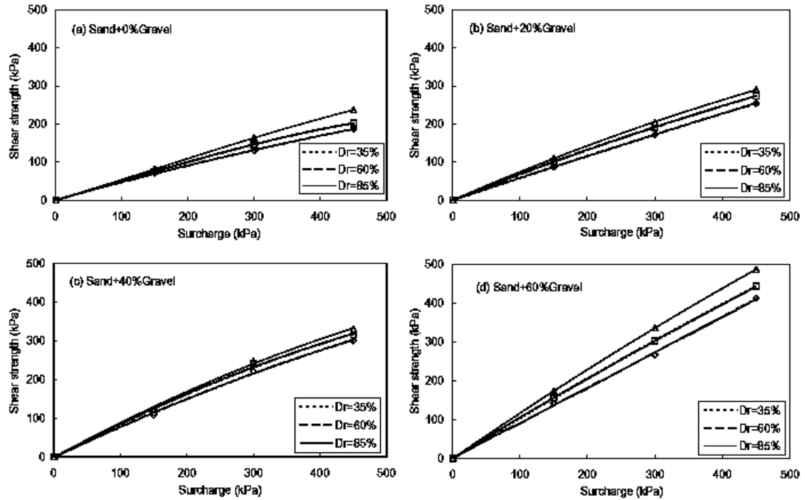
Fig.13 Failure envelope of sand-gravel mixtures in different relative densities
