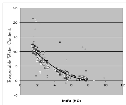
Fig. 2 The calibration curve of moisture meters.
