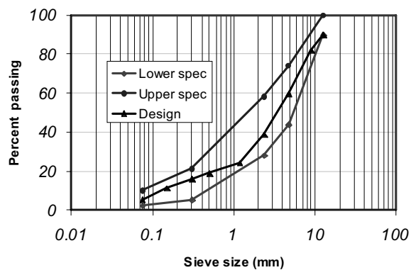
Fig. 2 Aggregate gradation used in asphalt concrete
