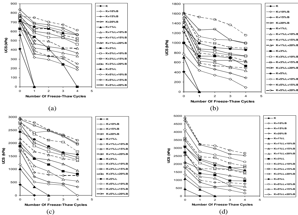
Fig. 6. UCS versus Number of freeze - thaw cycles for untreated, lime treated, BOS slag treated and BOS slag/lime treated kaolinite cured for (a) 1-day, (b) 7-days, (c) 28-days, (d) 90-days
