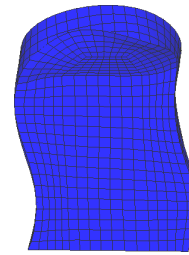
4-2: 1 st coupled mode Tank3 (T = 0.052 sec)
