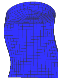
4-6: 2 nd coupled mode Tank3 (T = 0.037 sec)
