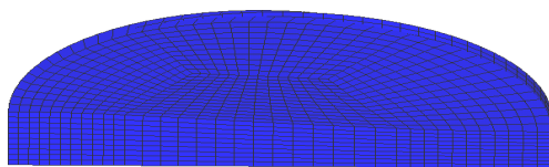
4-5: 1 st sloshing mode Tank3 (T = 2.475 sec)
