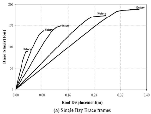
Fig. 6. Roof displacement-base shear curve for conventional X-brace
