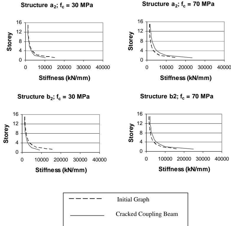
Fig. 7. Stiffness of the structures including coupled shear walls and the obligations of the American code
