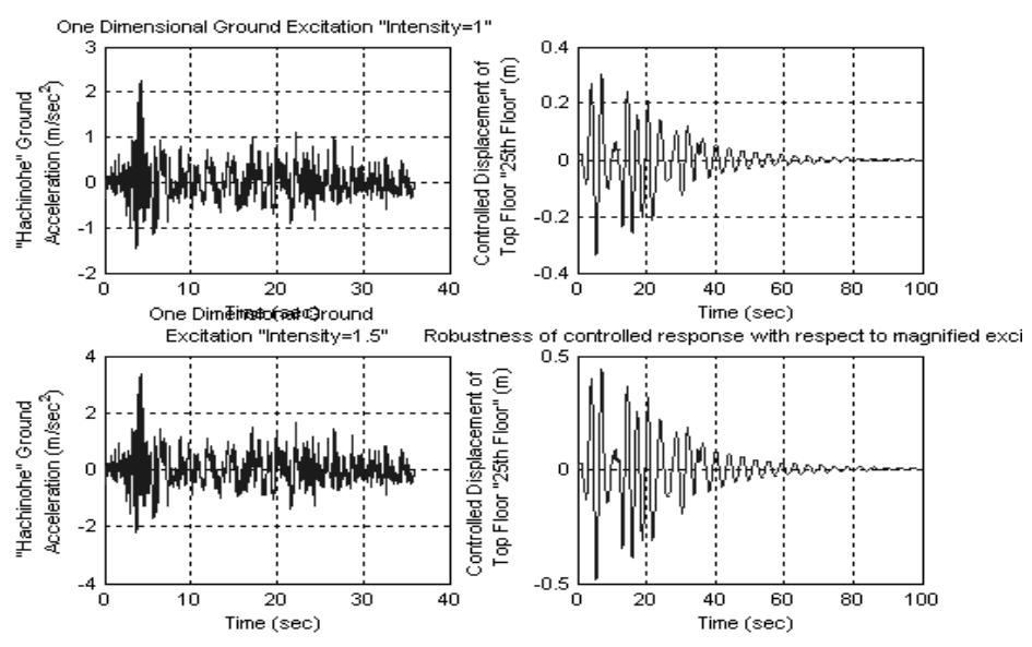
Fig.4 Assessment of control robustness of proposed Algorithm with respect to amplification of seismic Excitation. (Hachinohe Earthquake, Intensity=1 and Intensity=1.5).
