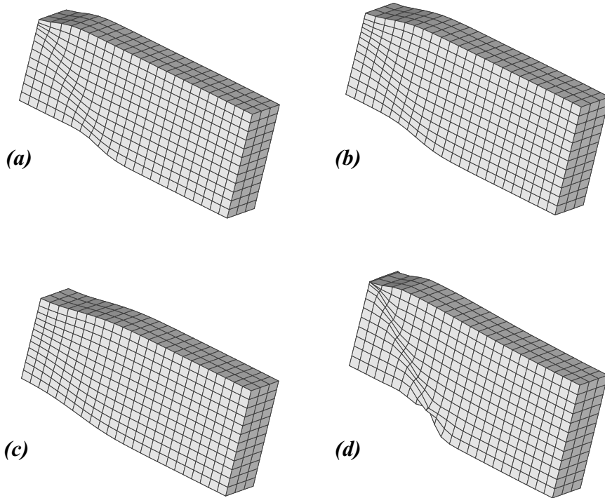
Figure 6. The deformed meshes of 3D (24x12x3) analyses for a strip in tensile using Cosserat theory at u = 4.2\text{mm} ; a) l_b = 1\text{mm} , l_t = 0 b) l_b = 2\text{mm} , l_t = 0 c) l_b = 3\text{mm} , l_t = 0 d) The classical theory
