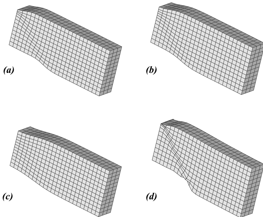
Figure 6. The deformed meshes of 3D (24x12x3) analyses for a strip in tensile using Cosserat theory at u = 4.2\text{mm} ; a) l_b = 1\text{mm} , l_t = 0 b) l_b = 2\text{mm} , l_t = 0 , c) l_b = 3\text{mm} , l_t = 0 d) The classical theory
