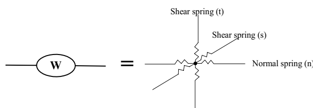
Fig. 2. Winkler spring in 3 dimensional state
