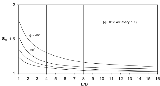
Fig. 22. Surcharge shape factors ( s_q ) for various \phi and L/B
