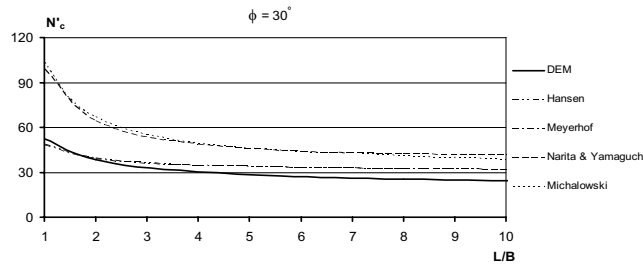
Fig. 18. Comparison of N'_c obtained from various methods for \phi = 30^\circ
