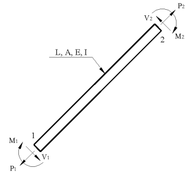
Fig. 1. Typical member of a frame
