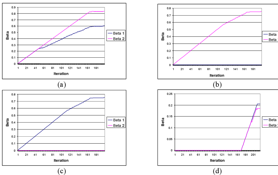
Fig. 3. Variation of design variables and during optimization process for each finite element (a) element 1 (b) element 2 (c) element 3 (d) element 4.
