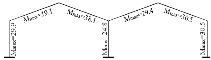
Fig. 12. Final maximum bending moments
