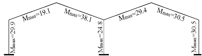
Fig. 12. Final maximum bending moments
