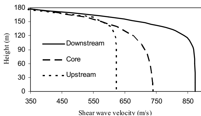
Fig. 3. Profile of shear wave velocity in the dam body (m/s) [18]
