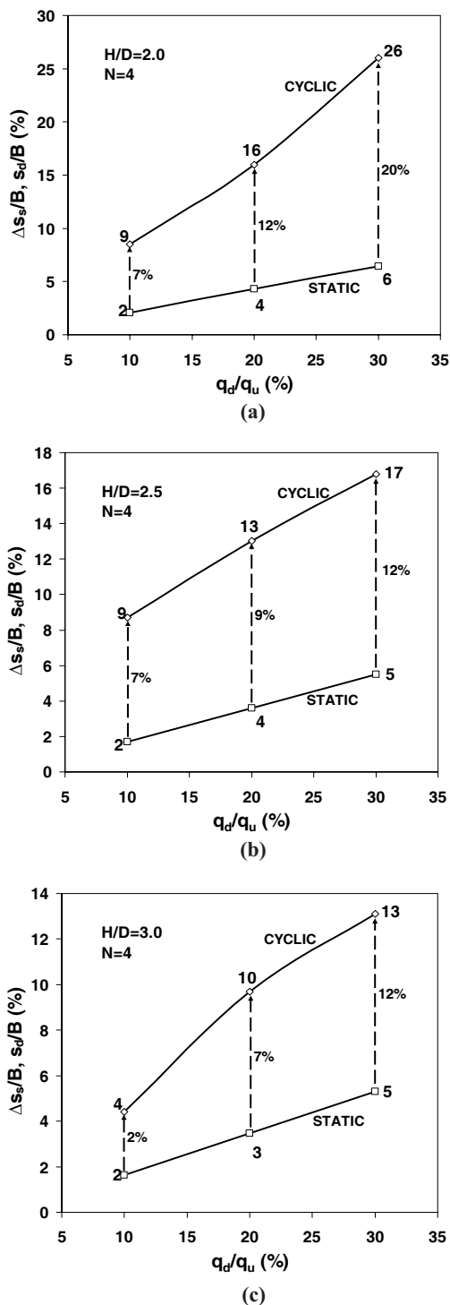
Fig. 17. Variation of cyclic footing settlement and static footing settlement versus the same amount of cyclic and static load of footing on 4 layers reinforced sand, (a) H/D=2.0 , (b) H/D=2.5 , (c) H/D=3.0
