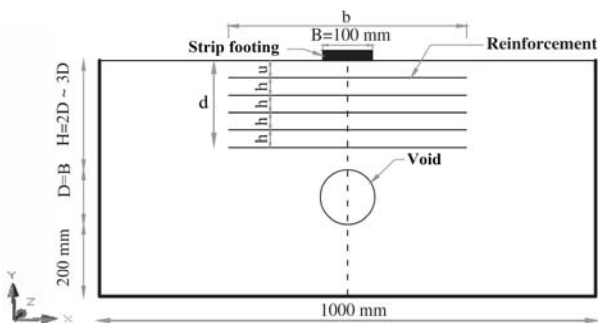
Fig. 2. View layout of trench (not in scale)
