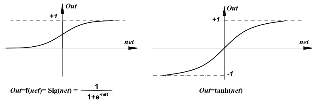
Fig. 3. Activation functions
