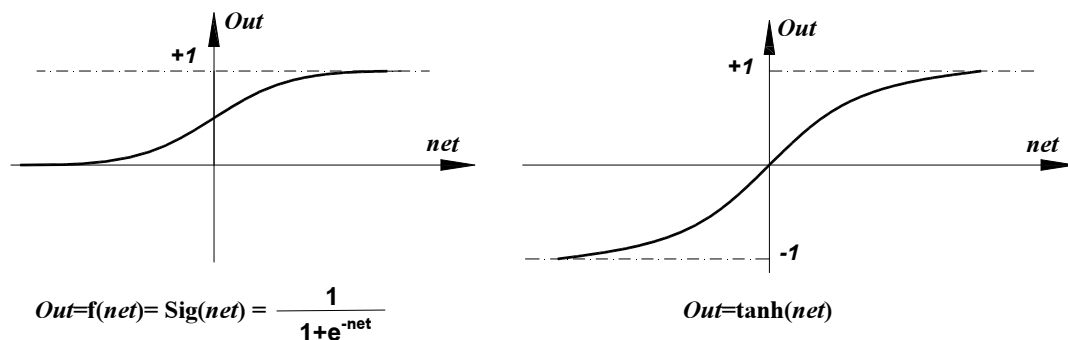
Fig. 3. Activation functions
