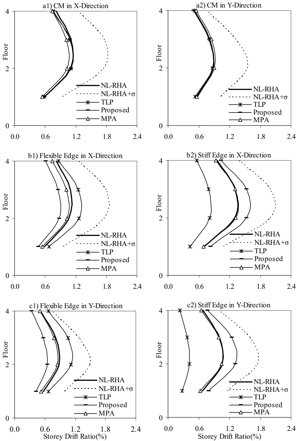
Fig. 8 Height-wise variation of the storey drifts for the torsionally-flexible 4-story building: a) at the CM; b) at the flexible and stiff edges in X-direction; and c) at the flexible and stiff edges in Y-direction
