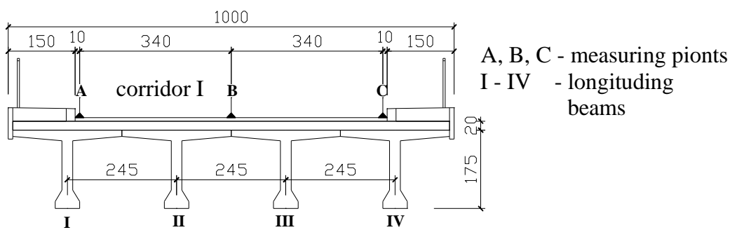
Fig. 4 The Brod bridge cross-section
