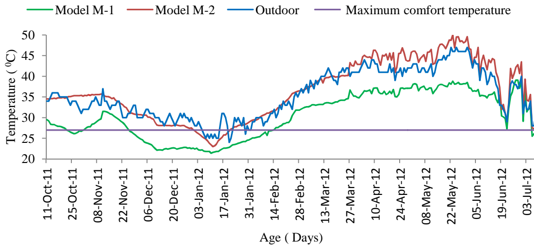
Fig. 4 Variation of maximum indoor temperature of model houses
