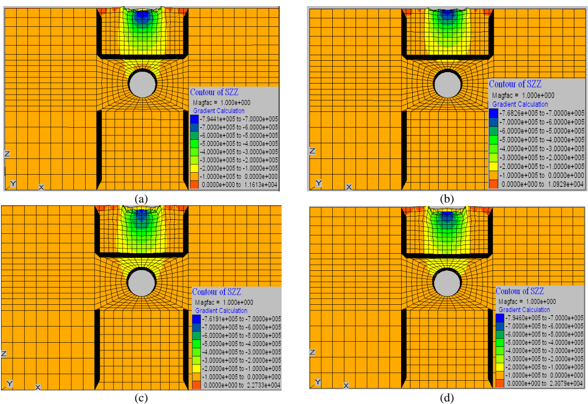
Fig. 10 Vertical stress contours obtained from numerical results for a) Soil Only (Ur) b) Soil Only (Re) c) C(5%)O-Ur, and d) C(5%)W-Ur
