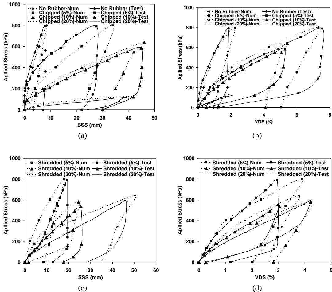
Fig. 6 Comparison between numerical and experimental results at calibration stage (a) SSS values for chipped rubbers, (b) VDS values for chipped rubbers, (c) SSS values for shredded rubbers, (d) VDS values for shredded rubbers
