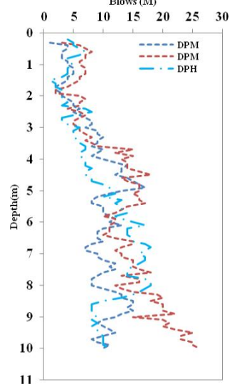
Fig. 2f Dynamic Probe depth profile from Rajae port
