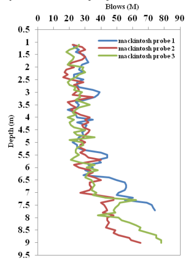
Fig. 2c Dynamic Probe depth profile from Emam khomeyni port
