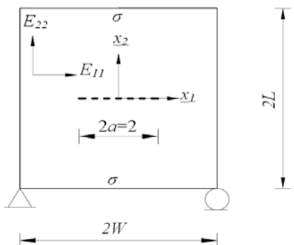
Fig.4 Geometry of the anisotropic tensile plate.
