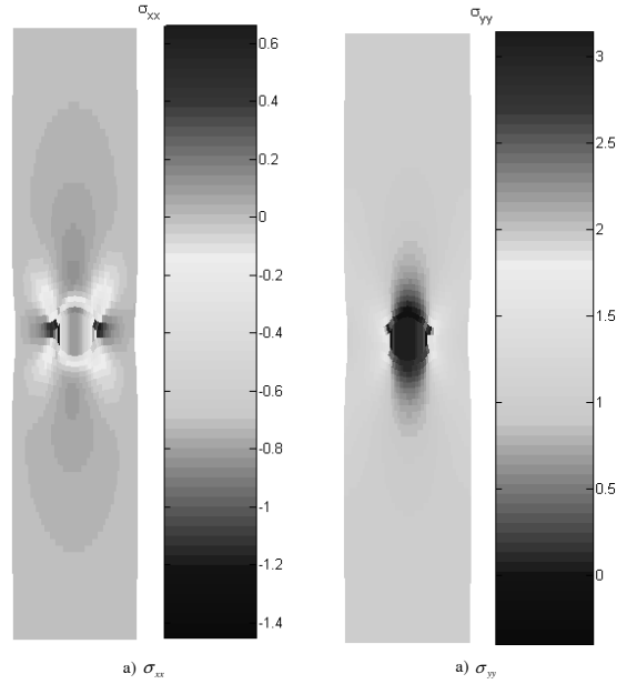
Fig. 8 Stress distribution
