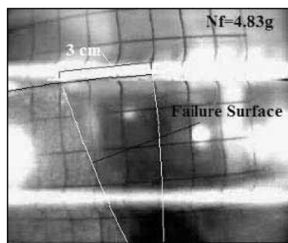
Fig. 7 Failure Surface in model No.2 ( N_f = failure acceleration in g)
