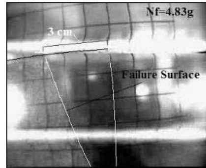
Fig. 7 Failure Surface in model No.2 ( N_f = 4.83g failure acceleration in g)
