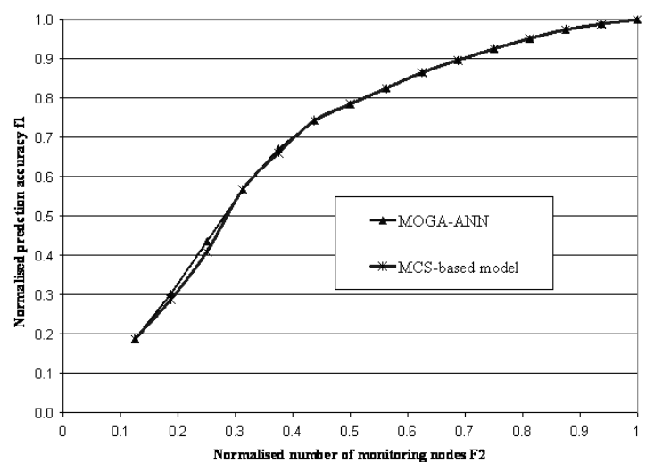
Fig. 6 Comparison of Pareto optimal fronts between MOGA-ANN and MCS-based model
