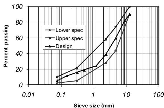
Fig. 2 Aggregate gradation used in asphalt concrete
