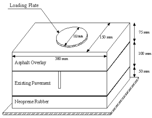
Fig. 1 Schematic of test set up
