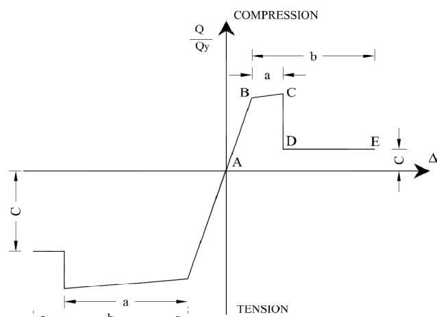
Fig. 1. Generalized force-deformation relation for steel brace elements (FEMA-356) [3].
