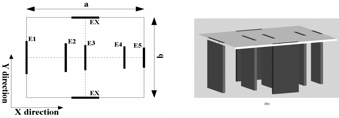
(a) Fig.4 arrangement of resisting element in (a) plan and (b) three dimension
