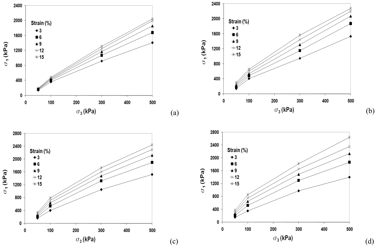
Fig.6 Strength values versus confining pressure for various number of reinforcement at different strain levels (a) N=1; (b) N=2; (c) N=3; and (d) N=4
