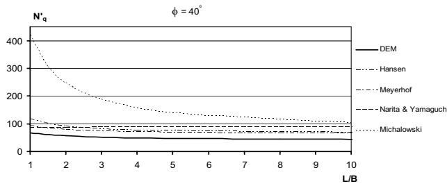
Fig. 17. Comparison of N'_q obtained from various methods for \phi = 40^\circ
