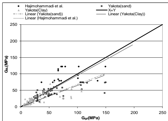
Fig. 7. Comparison between shear modulus obtained from present study and those obtained by Yokota & Kanno (1985) [29]
