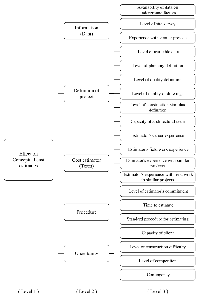
Fig. 2. Structure hierarchy
