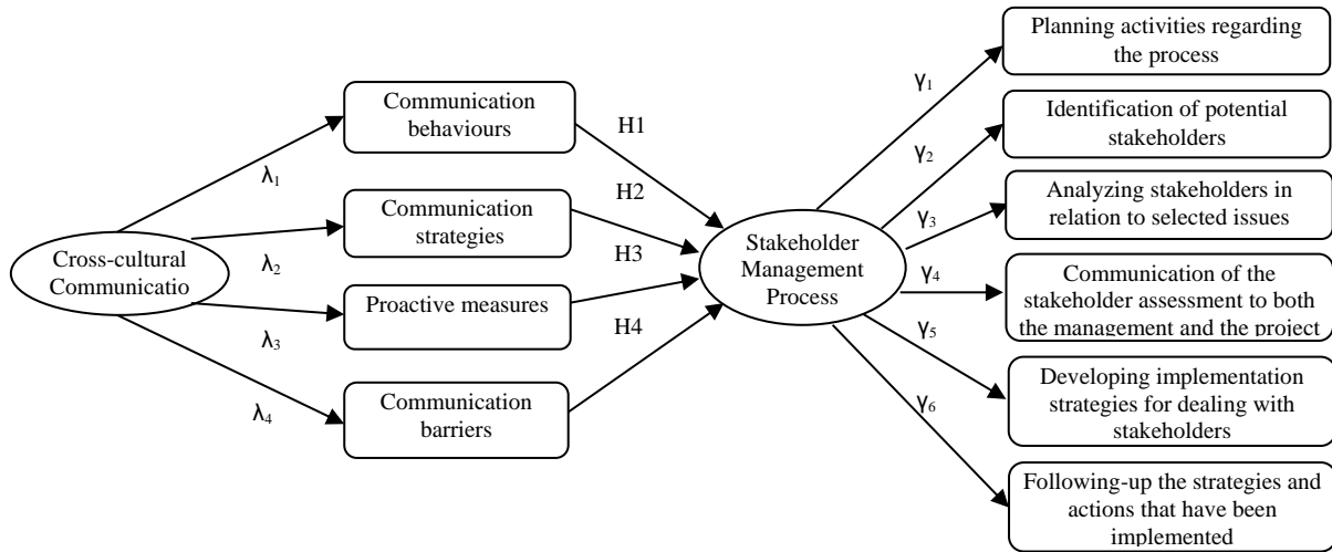
Fig. 1 Hypothesized model
