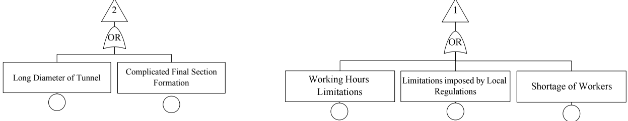
Fig. 3 b- Subtrees 1 and 2 of fault tree presented in Fig. 3-a
