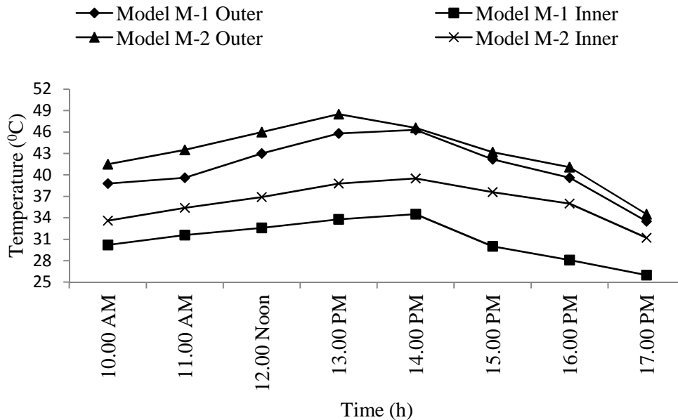
Fig. 7 Variations of the outside and inside surface temperatures of south side wall for the waste-create brick model house and the fly ash brick model house (11 th October 2011)
