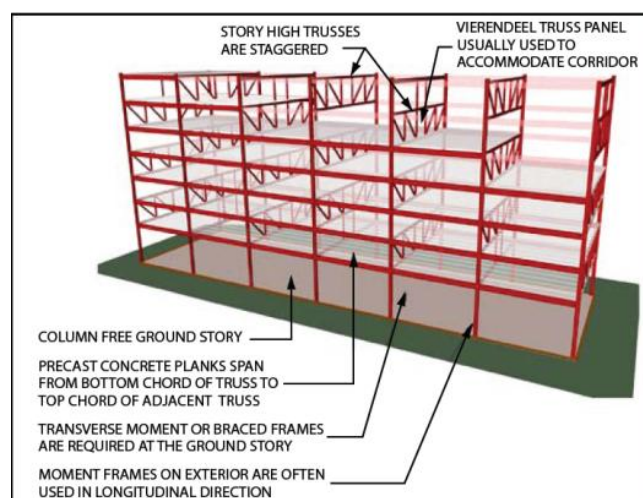
Fig. 1 Staggered Truss Framing System [1, 7]
