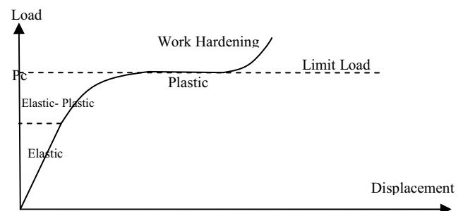
Fig. 1. Load-displacement curve
