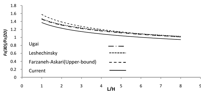
Fig. 14. Comparison with those of Ugai, Leshchonsky, Farzaneh-Askari in cohesive soil
