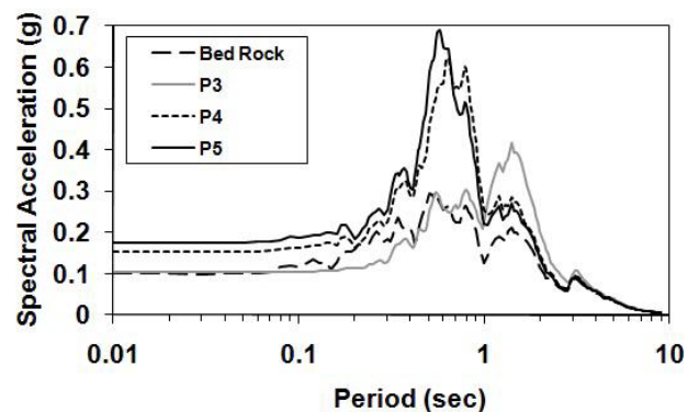
Fig. 15 S_a of P3, P4, and P5 for Chichi
