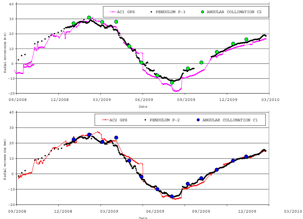
Fig. 8 Comparison of monitoring results: DGPS, pendulums and angular collimation
