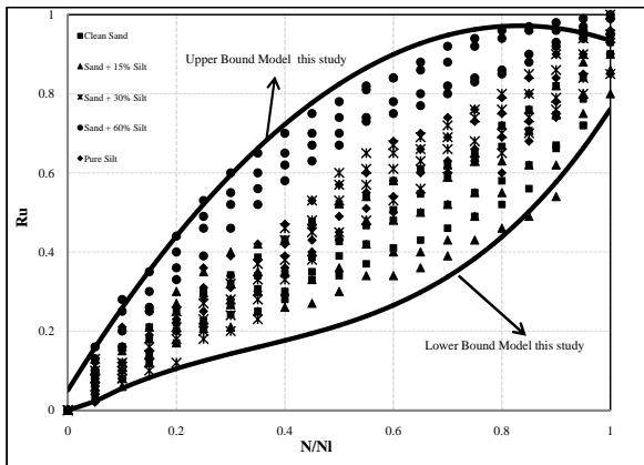
Fig. 15. Excess pore water pressure generation data for all specimens and comparison with model presented in this study.
