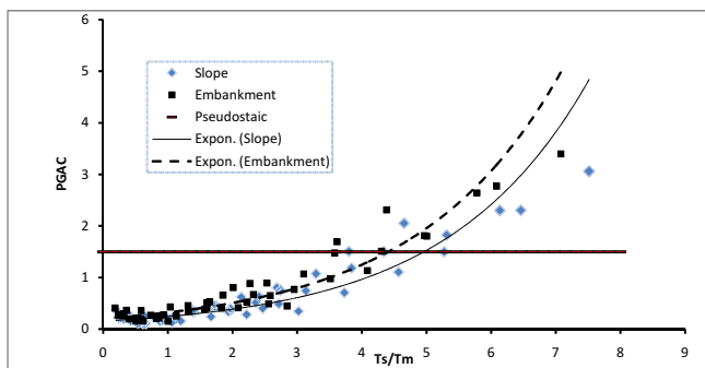
Fig. 6. Pseudostatic and shakedown critical PGAC against variation in T_s/T_m for slope and embankment examples presented in this study ( \gamma H/c=4 , \varphi=30^\circ and DR=5\% )
