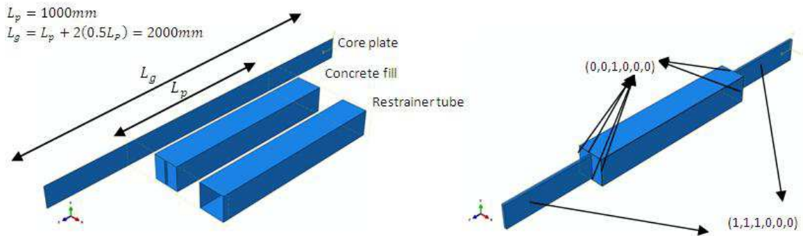
Fig. 2 overall schematic of group A of models
