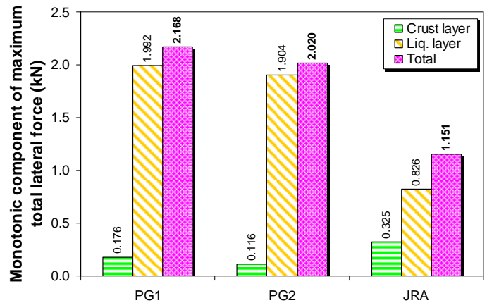
Fig. 13 Comparison between monotonic components of maximum total lateral forces in different pile groups from this experiment and JRA [27] recommended values
