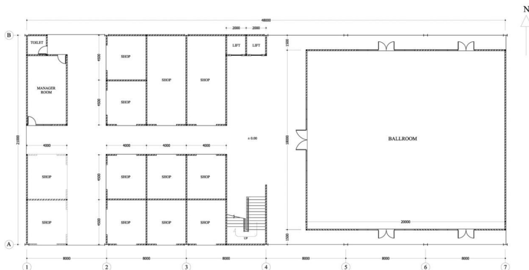
FIRST FLOOR PLAN 1:250
