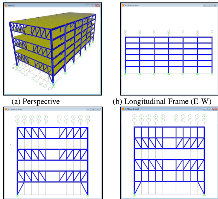
(a) Perspective (b) Longitudinal Frame (E-W) (c) Transverse Frame, Odd Axis (N-S) (d) Transverse Frame, Even Axis (N-S) Fig. 4 Building Modeling With STF System
