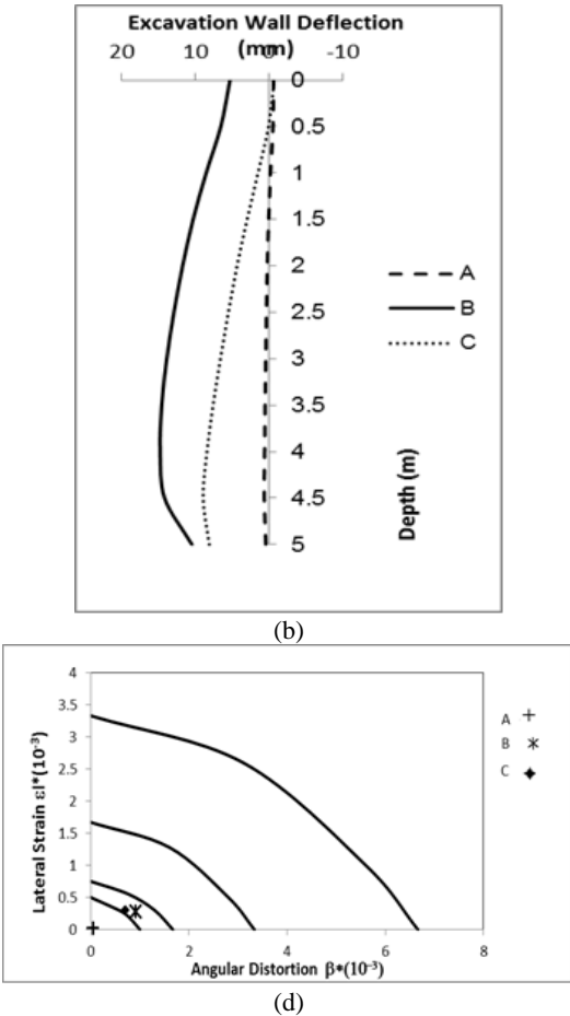
Fig. 12 (a) Ground surface settlement, (b) Deformation of excavation wall, (c) Strut stress during excavation procedure, (d) Deflection parameters of building in Boscardin and Cording diagram
