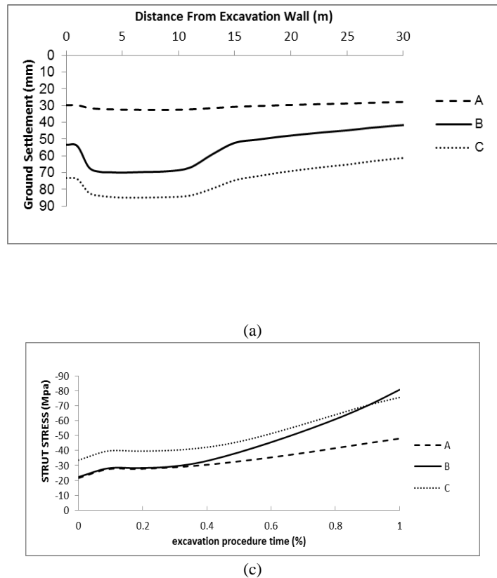
Fig. 12 (a) Ground surface settlement, (b) Deformation of excavation wall, (c) Strut stress during excavation procedure, (d) Deflection parameters of building in Boscardin and Cording diagram
