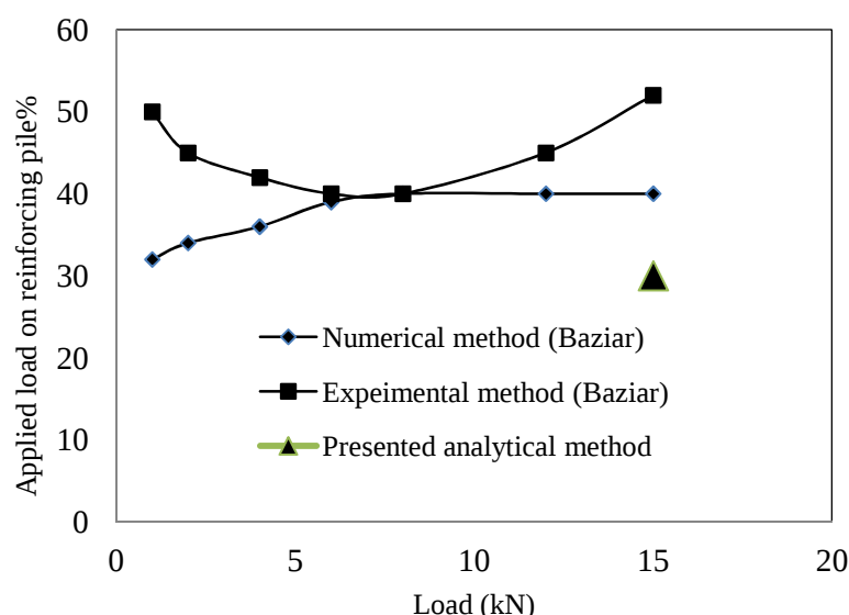
Fig. 12 Comparing suggested method with experimental and numerical method presented with Baziar, et. al to determine percent of applied load on pile
