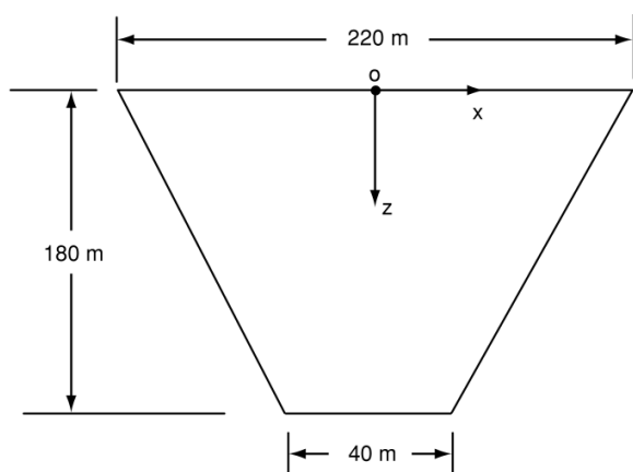
Fig. 5 The valley dimensions of the arch dam
