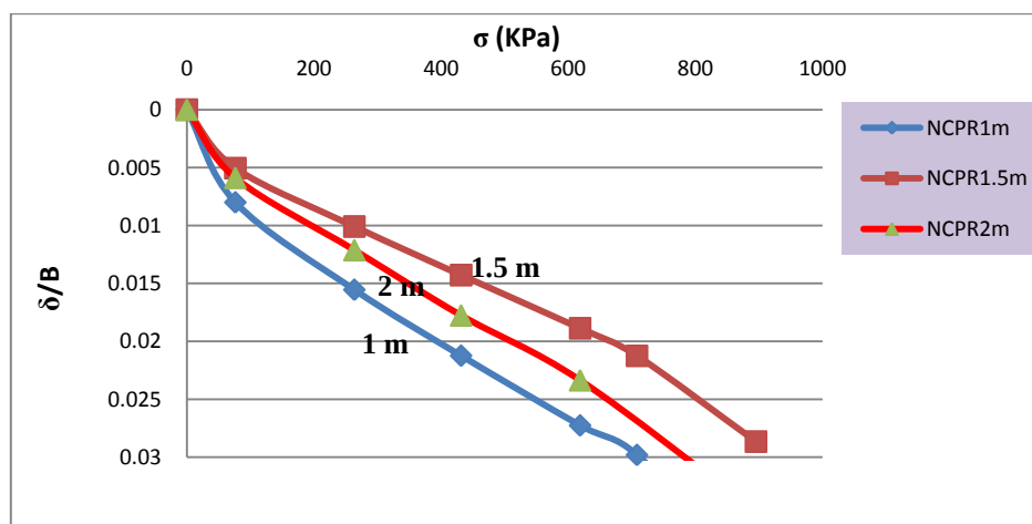
Fig. 5 The load settlement curve for non-connected pile raft system using layers with 1, 1.5 and 2cm thickness
