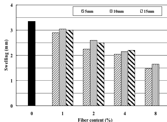
Fig. 4 Variations of swelling with fiber content and length.
