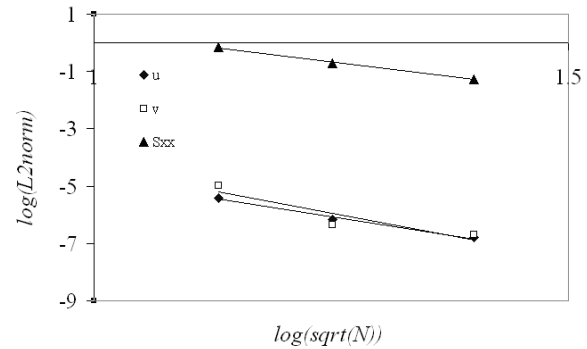
Figure 13 The convergence rate of the infinite plate with a circular hole. a) H^1 error norm and b) L^2 error norm of displacements and normal stress
