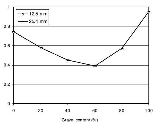
Fig.2 Maximum and minimum void ratios of different mixtures
