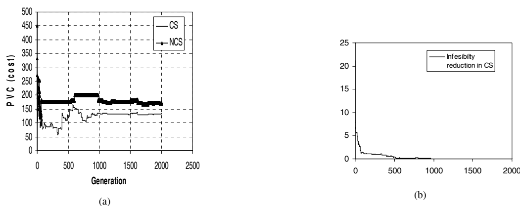
Fig. 5 GA procedure (a) Convergency curves in CS and NCS for best computed run (b) Infeasibility accompanied in CS
